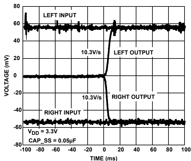
FIGURE 29. SOFT-START (0.05 \mu\text{F} ) CLICK/POP REDUCTION
