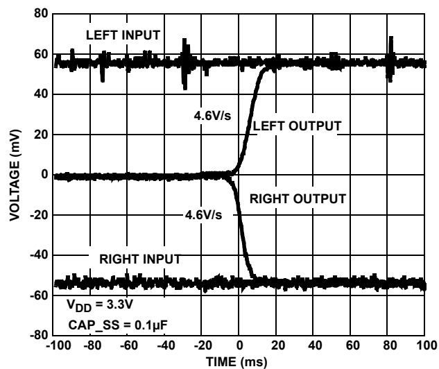
FIGURE 28. SOFT-START (0.1 \mu\text{F} ) CLICK/POP REDUCTION
