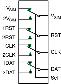
Figure 1. Analog Symbol
