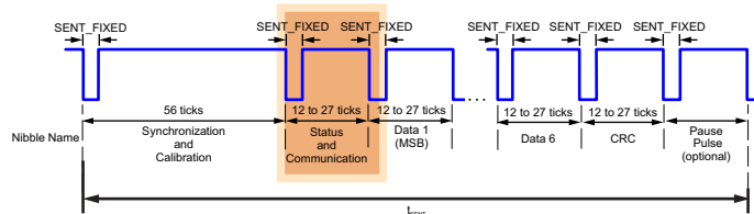
Figure 11: SCN Nibble in SENT Message
