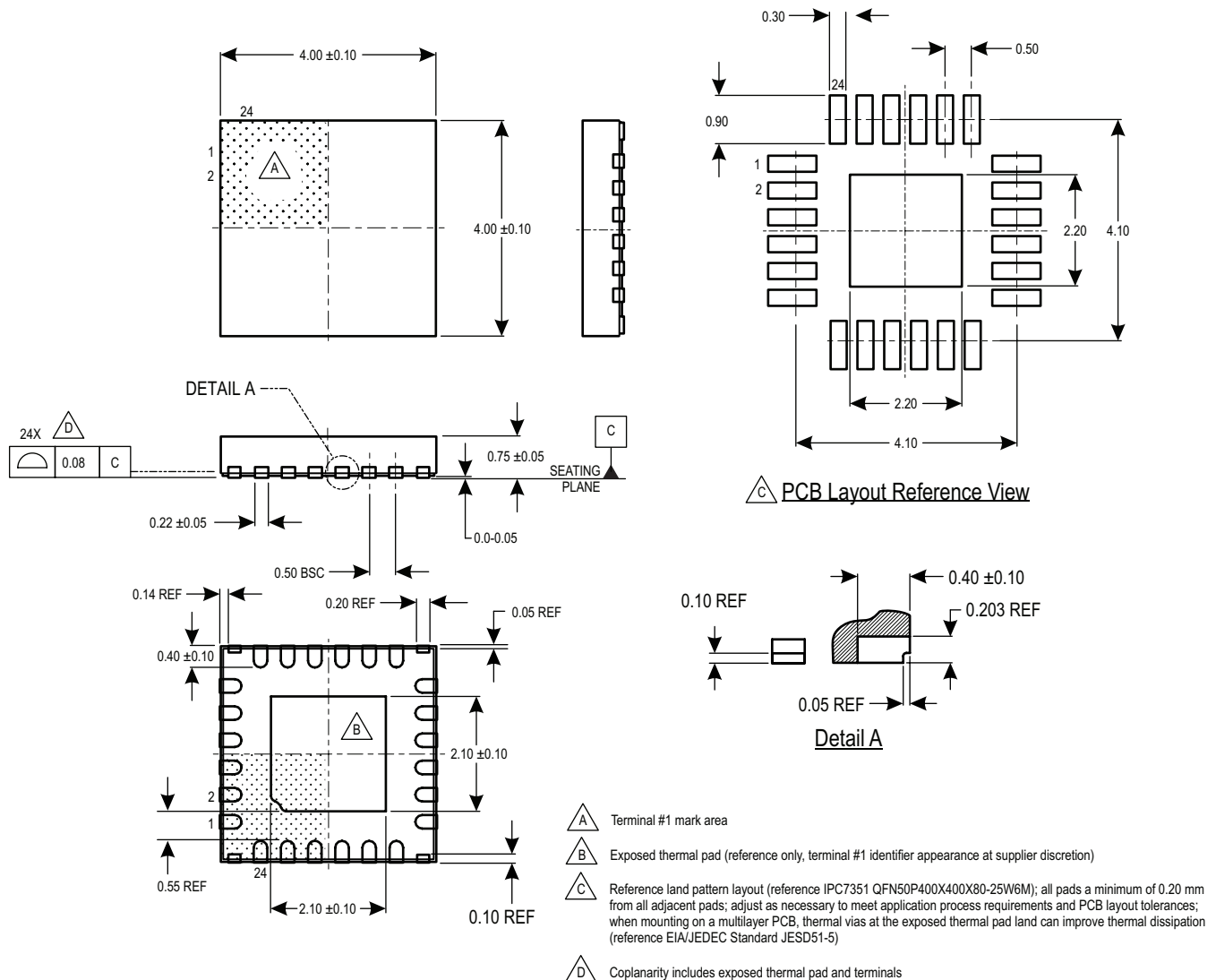
Figure 21: Package ES, 24-pin wettable flank QFN with exposed thermal pad
