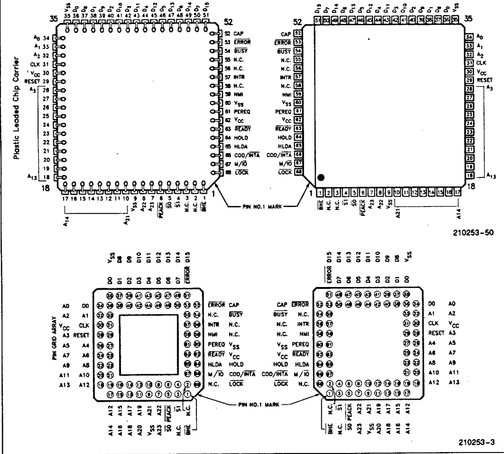
Figure 2. 80286 Pin Configuration
