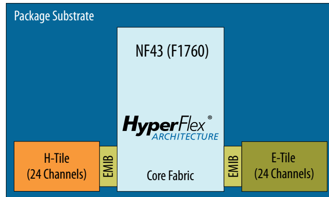
Figure 4. Tile Configuration 2: NF43 Package
