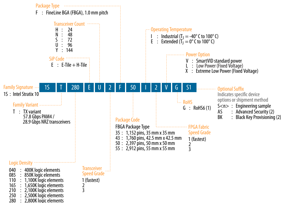
Figure 1. Sample Ordering Code and Available Options for Intel Stratix 10 TX Devices
