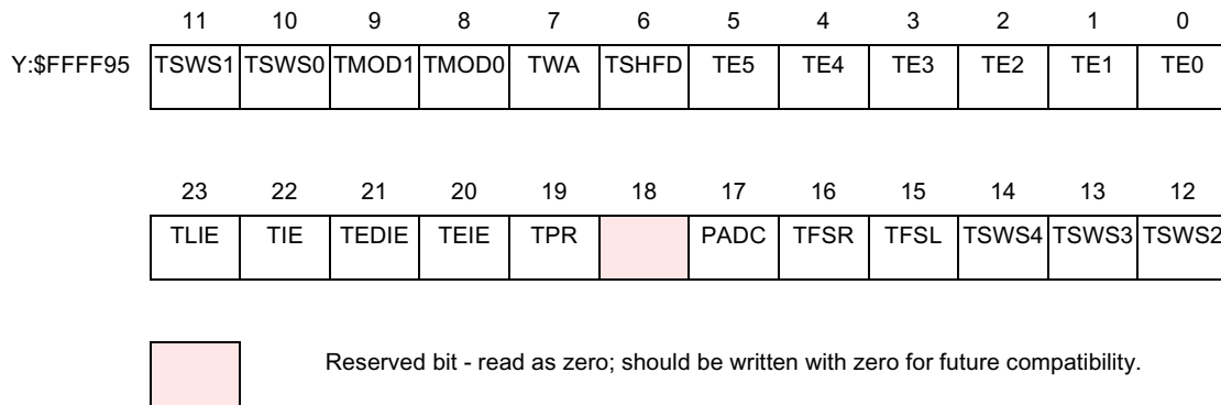
Figure 11-6 TCR_1 Register
