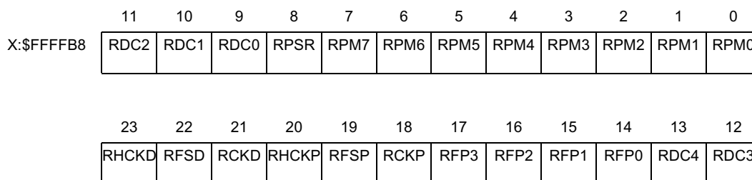
Figure 10-8 RCCR Register
