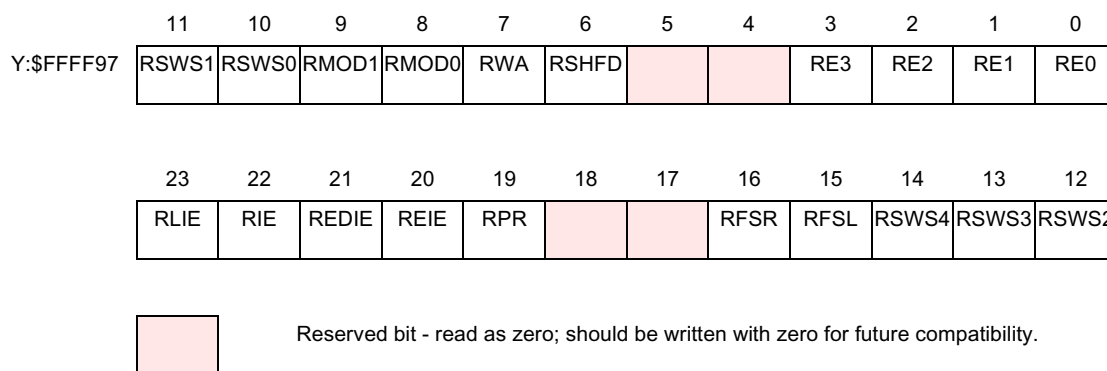
Figure 11-8 RCR_1 Register
