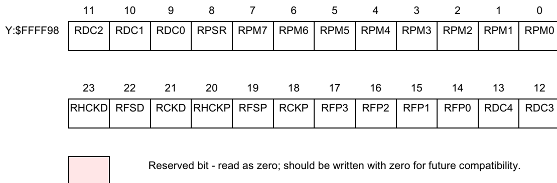
Figure 11-7 RCCR_1 Register
