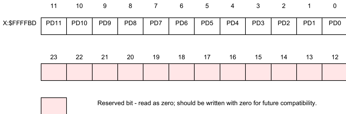
Figure 10-21 PDRC Register
