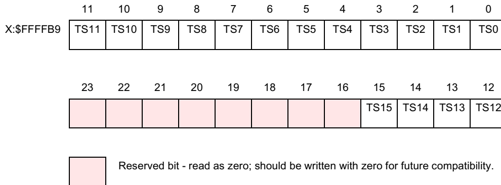
Figure 10-15 TSMA Register
