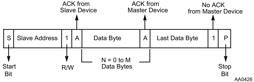
Figure 9-11 I 2 C Bus Protocol For Host Read Cycle
