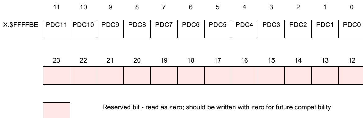
Figure 10-20 PRRC Register
