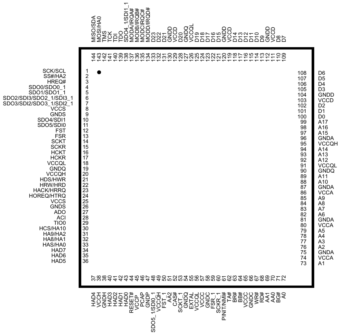
Figure 14-1 144-pin package
