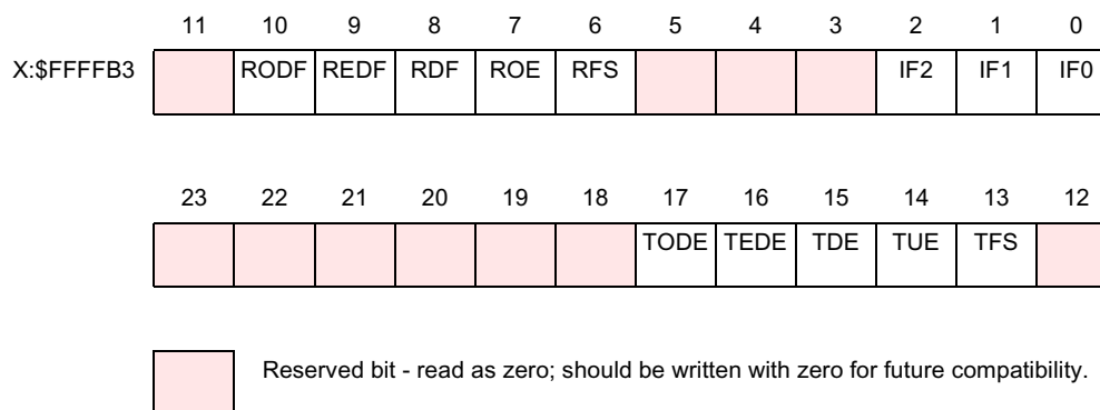
Figure 10-12 SAISR Register
