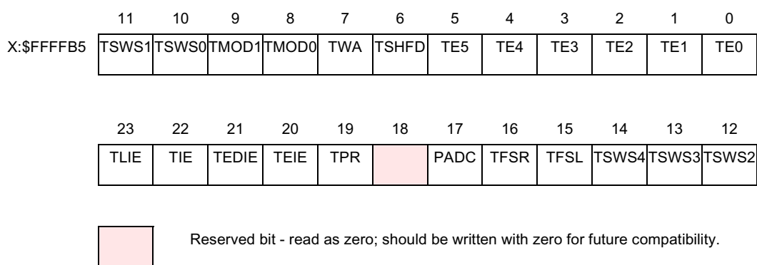
Figure 10-5 TCR Register
