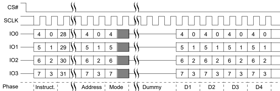
Figure 69. Quad I/O Read Command Seq. (4-Byte Address, ECh or EBh [CR2V[7]=1]) QPI Mode
