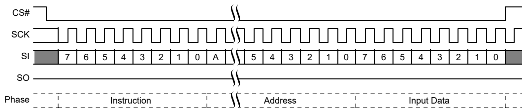
Figure 91. DYBWR Command Sequence [59, 60]
