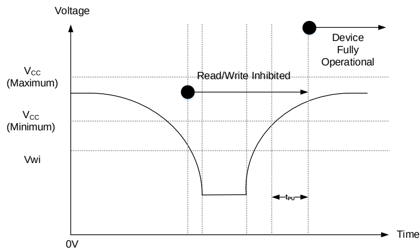
Figure 5: Power-Down Behavior
