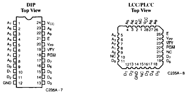
Figure 1. Programming Pinouts
