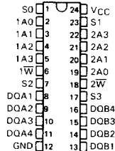
SN54AS871 . . . JD PACKAGE SN74AS871 . . . N PACKAGE
