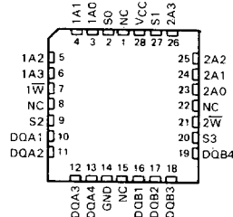
SN54AS871 . . . FK PACKAGE SN74AS871 . . . FN PACKAGE
