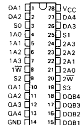
SN54AS870 . . . FK PACKAGE SN74AS870 . . . FN PACKAGE
