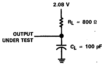
FIGURE 3. OUTPUT LOAD CIRCUIT
