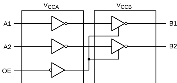
Figure 1. Logic Diagram
