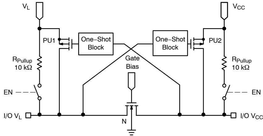
Figure 1. Block Diagram (1 I/O Line)
