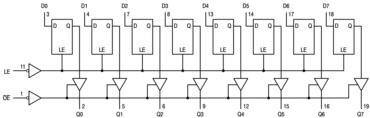
Figure 9. Expanded Logic Diagram
