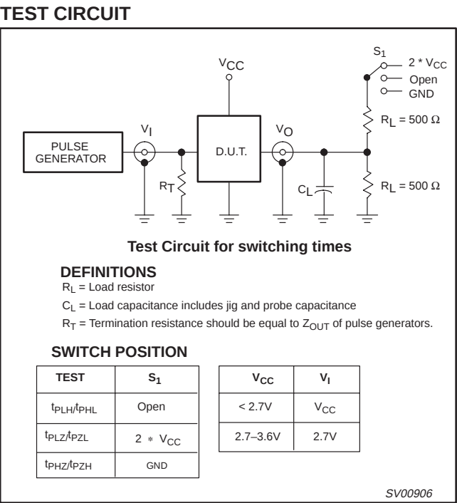
Waveform 3. Load circuitry for switching times
