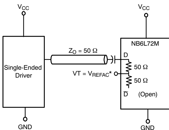
Figure 14. Capacitor-Coupled Single-Ended Interface ( V_T Connected to V_{REFAC} )
