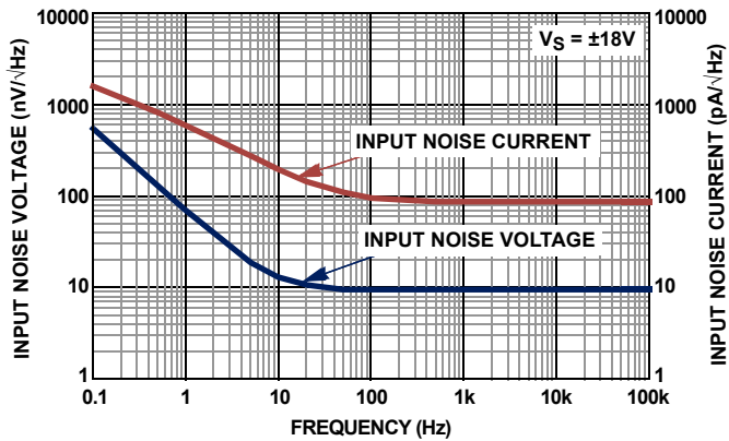
FIGURE 24. CHARACTERIZED INPUT NOISE VOLTAGE
