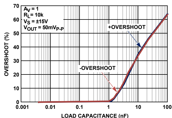
FIGURE 14. OVERSHOOT vs LOAD CAPACITANCE
