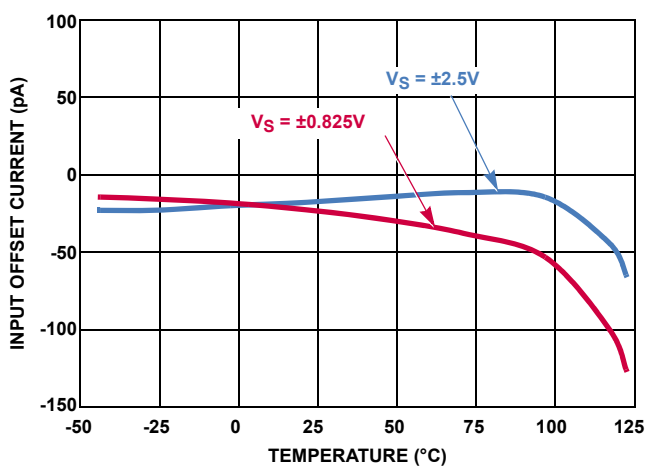
FIGURE 6. I_{OS} vs TEMPERATURE
