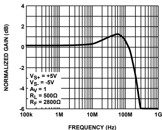
FIGURE 2. FREQUENCY RESPONSE ( A_V = +1 )
