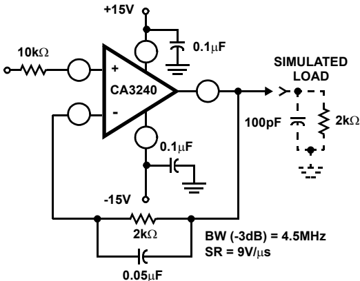
FIGURE 1C. TEST CIRCUIT
