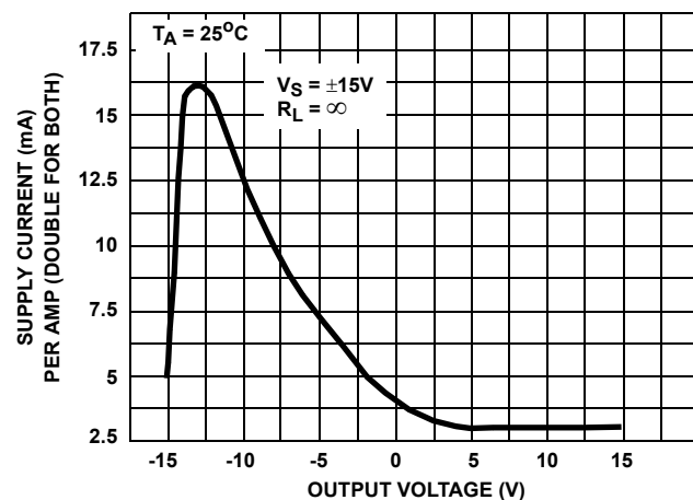
FIGURE 21. SUPPLY CURRENT vs OUTPUT VOLTAGE
