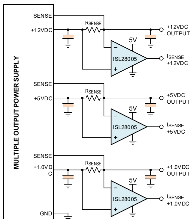
Figure 1. Typical Application
