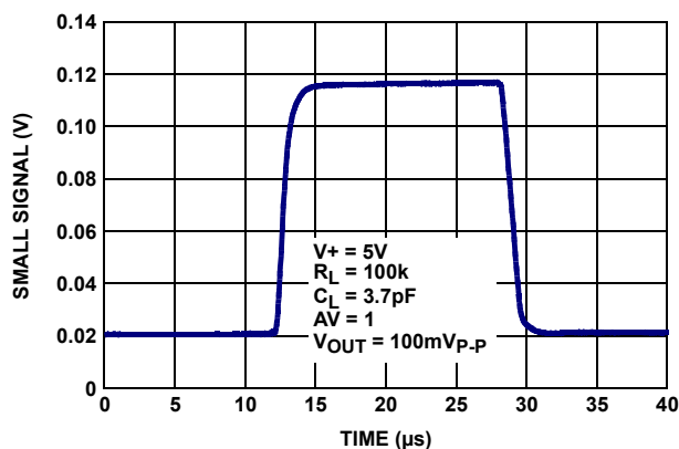
FIGURE 32. SMALL SIGNAL STEP RESPONSE (100mV)
