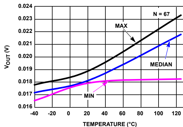
FIGURE 34. V_{OUT} LOW vs TEMPERATURE, R_L = 10k , V_S = 5V
