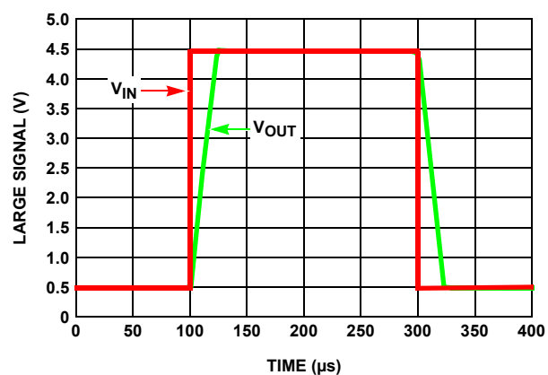
FIGURE 50. SIMULATED LARGE SIGNAL STEP RESPONSE (4V)
