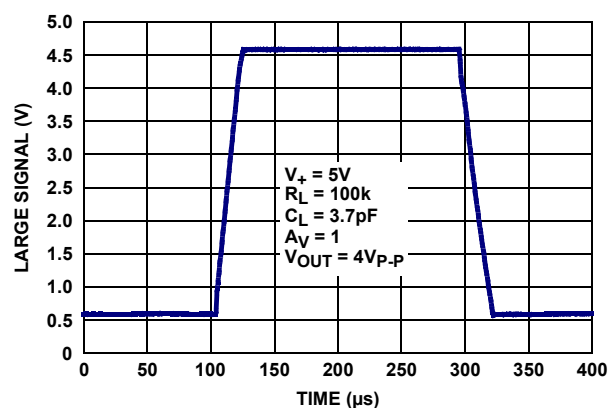
FIGURE 30. LARGE SIGNAL STEP RESPONSE (4V)
