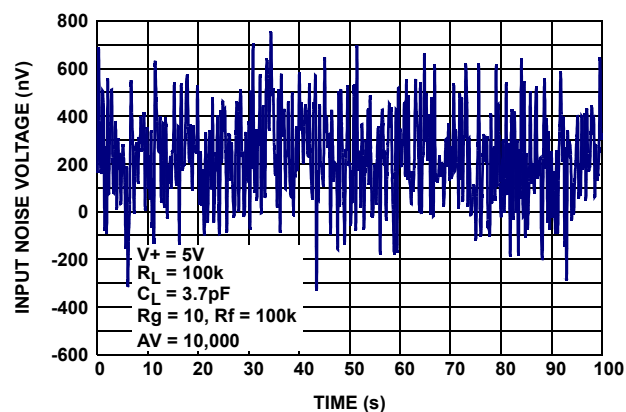
FIGURE 12. INPUT NOISE VOLTAGE 0.01Hz TO 10Hz
