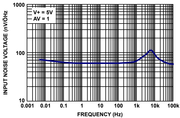
FIGURE 43. CHARACTERIZED INPUT NOISE VOLTAGE DENSITY vs FREQUENCY
