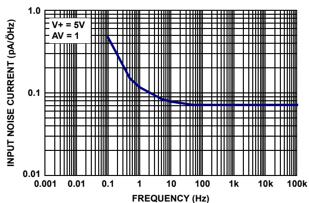
FIGURE 14. INPUT NOISE CURRENT DENSITY vs FREQUENCY
