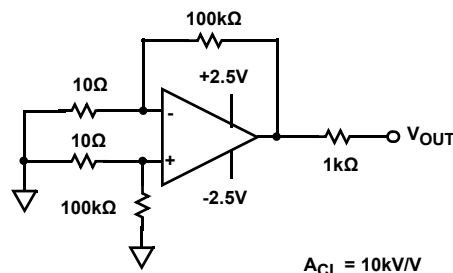
FIGURE 40. LONG TERM DRIFT TEST CIRCUIT
