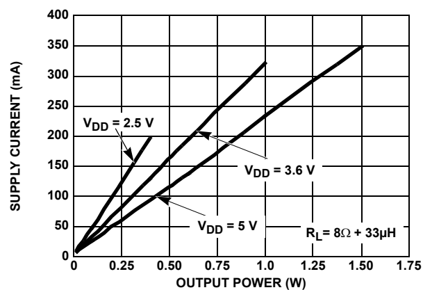
FIGURE 2. SUPPLY CURRENT vs OUTPUT POWER
