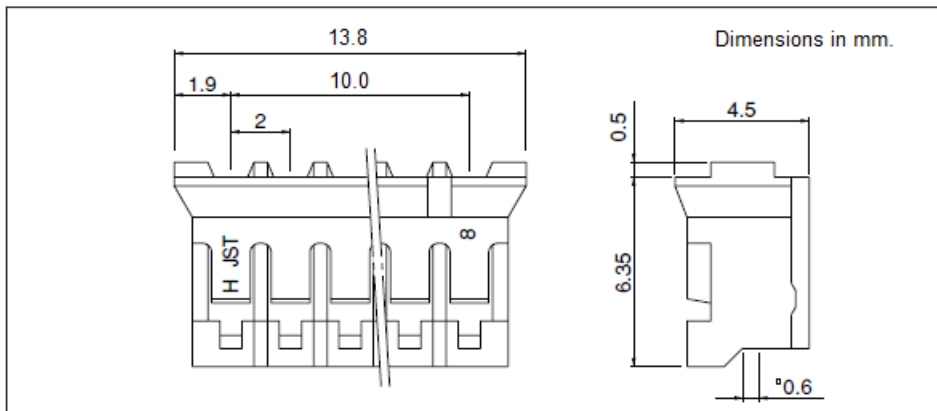
Figure 8. Receptacle Drawing
