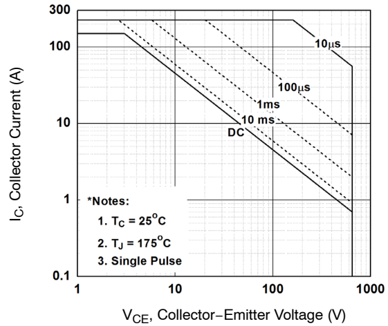
Figure 16. SOA Characteristics
