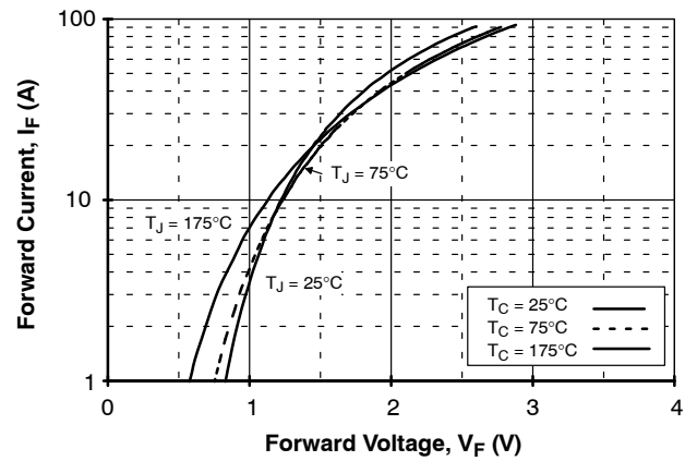
Figure 16. Forward Characteristics
