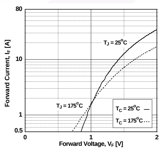
Figure 18. Forward Characteristics
