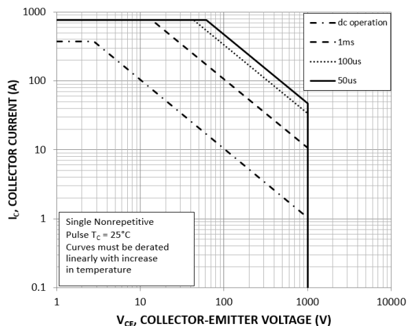
Figure 43. FBSOA – Outer IGBT
