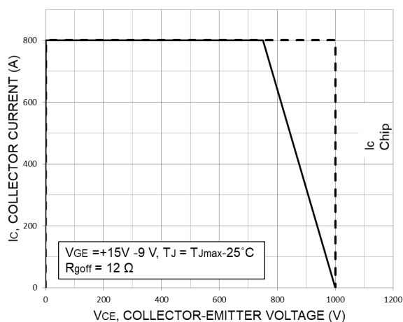
Figure 44. RBSOA – Outer IGBT
