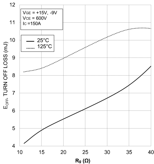
Figure 24. Typical Turn Off Loss vs. R_G
