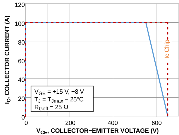
Figure 28. IGBT RBSOA
