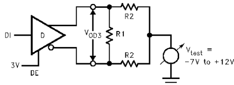
FIGURE 2. V_{OD3}
