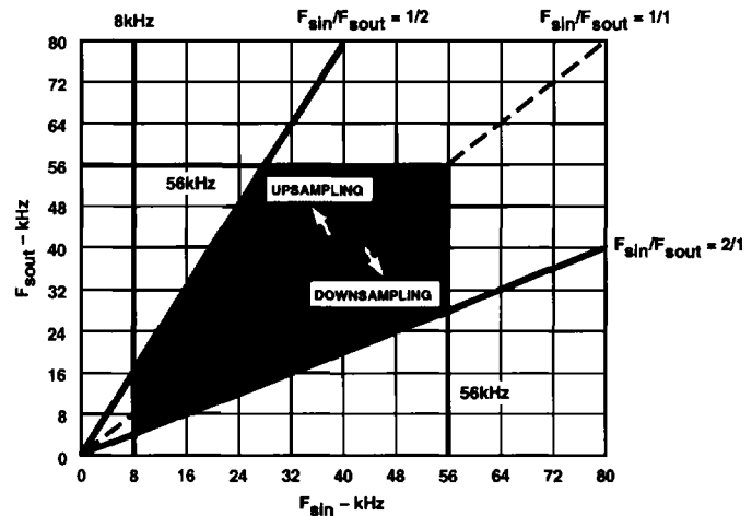
Figure 10. Allowable Input and Output Sample Frequencies MCLK = 16 MHz Case
