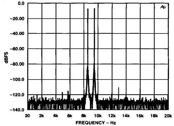
Figure 20b. AD1891—Twitone, 10 kHz and 11 kHz, 44.1 kHz Input Sample Frequency, 48 kHz Output Sample Frequency, 16k-Point FFT, BH4 Window
