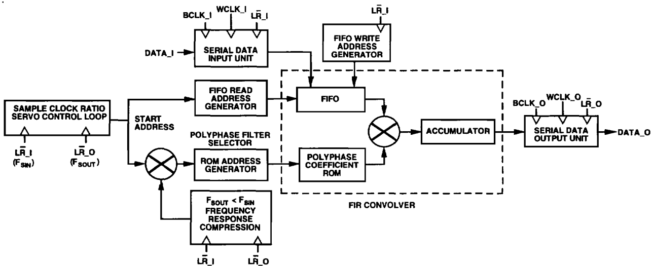
Figure 6. AD1890/AD1891 Functional Block Diagram
