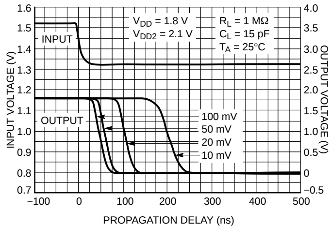
Figure 7. High to Low Propagation to DET with Changing Input Overdrive of L_DET
