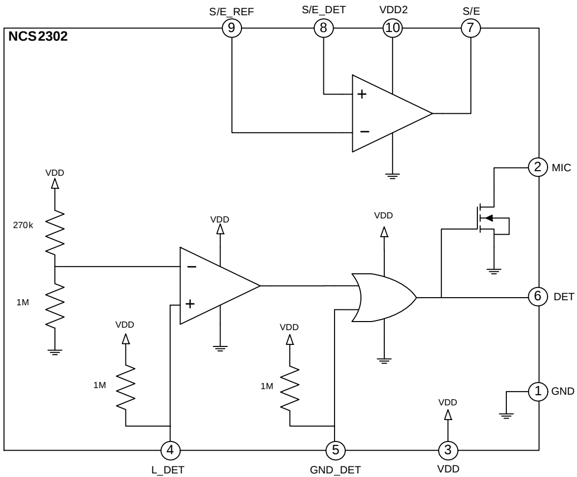
Figure 2. Block Diagram
