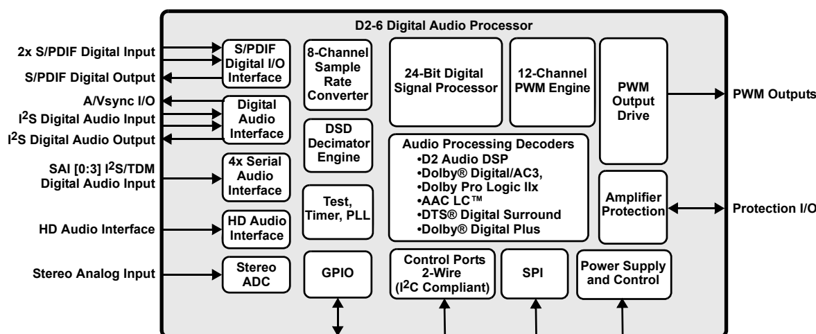
FIGURE 1. BLOCK DIAGRAM
