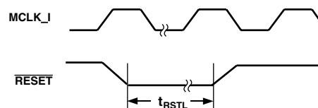
Figure 2. \overline{\text{RESET}} Timing
