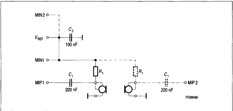
Figure 40 Interfacing Electret Microphones with Bias from V_{REF}
