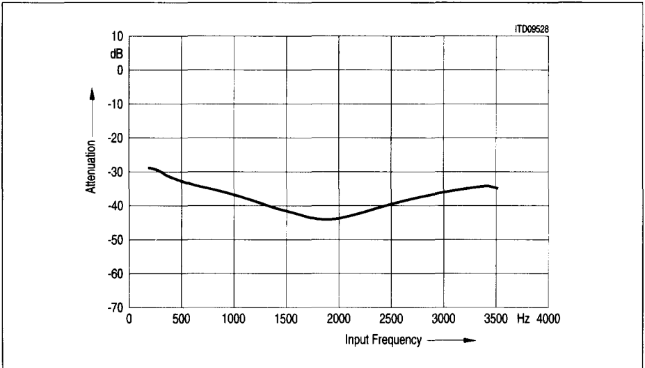
Figure 82 Transhybrid Loss
