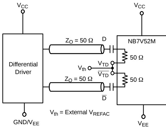
Figure 16. Capacitor-Coupled Differential Interface ( V_{TD}/\overline{V_{TD}} Connected to External V_{REFAC} ; V_{REFAC} Bypassed to Ground with 0.1\ \mu F Capacitor)
