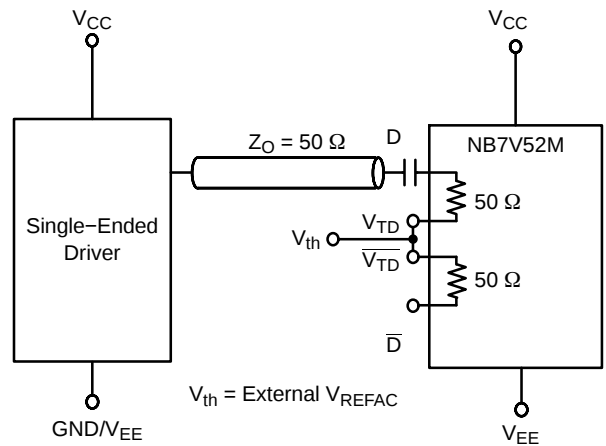
Figure 17. Capacitor-Coupled Single-Ended Interface ( V_{TD}/\overline{V_{TD}} Connected to External V_{REFAC} ; V_{REFAC} Bypassed to Ground with 0.1\ \mu F Capacitor)
