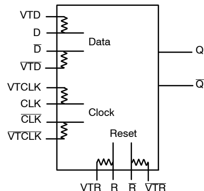
Figure 1. Logic Diagram
