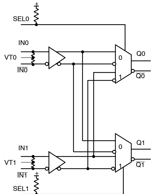
Figure 1. Logic Diagram
