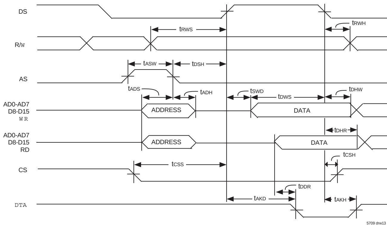
Figure 13. Multiplexed Bus Timing (Motorola Mode)
