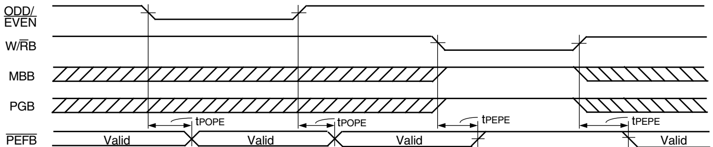
Figure 12. ODD/ \overline{\text{EVEN}} , W/RB, MBB, and PGB to \overline{\text{PEFB}} Timing
