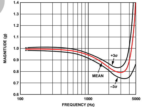
Figure 21. Magnitude/Frequency Response
