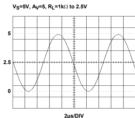
FIGURE 24. OUTPUT SWING
