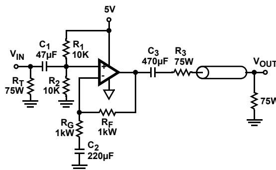
FIGURE 33. 5V SINGLE SUPPLY NON-INVERTING VIDEO LINE DRIVER
