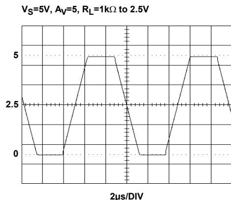
FIGURE 22. OUTPUT SWING
