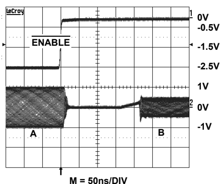
FIGURE 32. ENABLE SIGNAL
