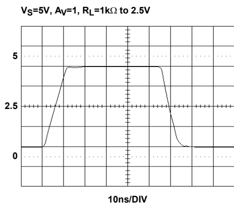
FIGURE 21. LARGE SIGNAL TRANSIENT RESPONSE
