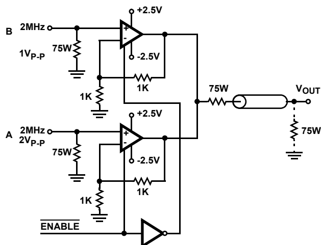
FIGURE 31. TWO TO ONE MULTIPLEXER
