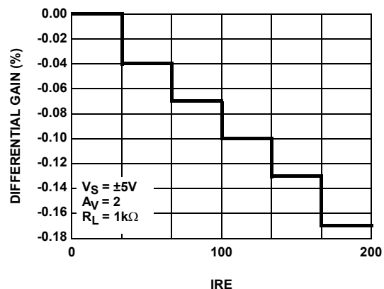
FIGURE 11. DIFFERENTIAL GAIN
