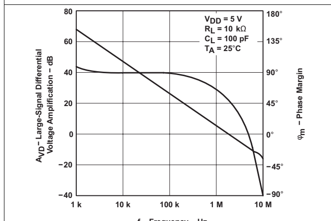
Figure 21. Large-Signal Differential Voltage Amplification and Phase Margin vs Frequency
