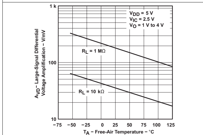
Figure 23. Large-Signal Differential Voltage Amplification vs Ambient Temperature
