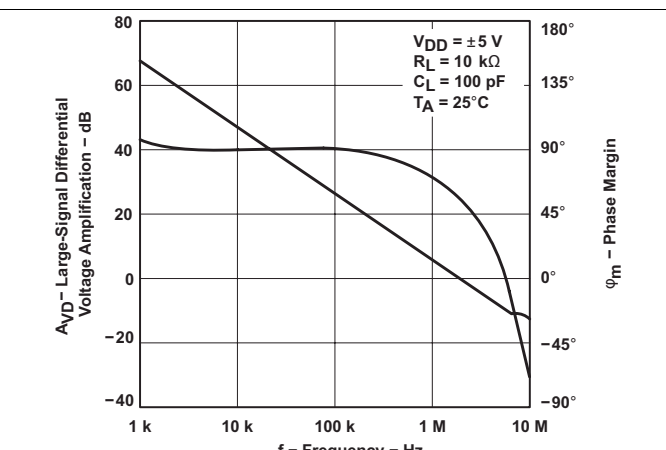
Figure 22. Large-Signal Differential Voltage Amplification and Phase Margin vs Frequency
