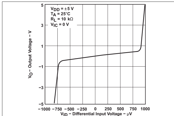
Figure 19. Output Voltage vs Differential Input Voltage
