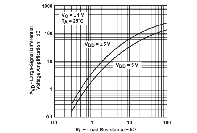
Figure 20. Large-Signal Differential Voltage Amplification vs Load Resistance
