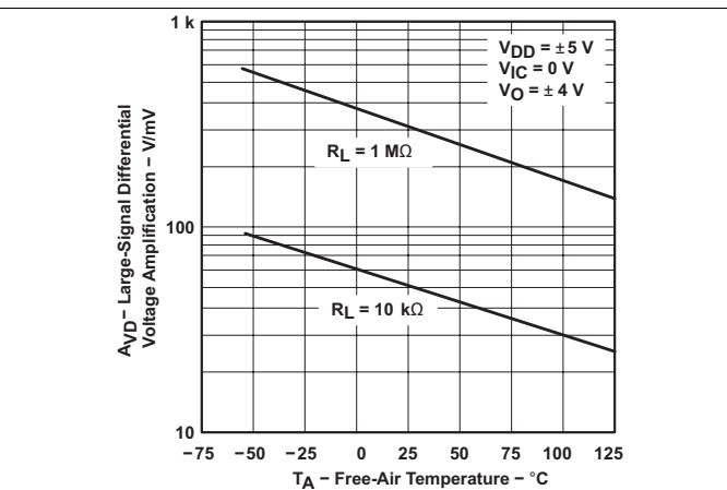
Figure 24. Large-Signal Differential Voltage Amplification vs Ambient Temperature
