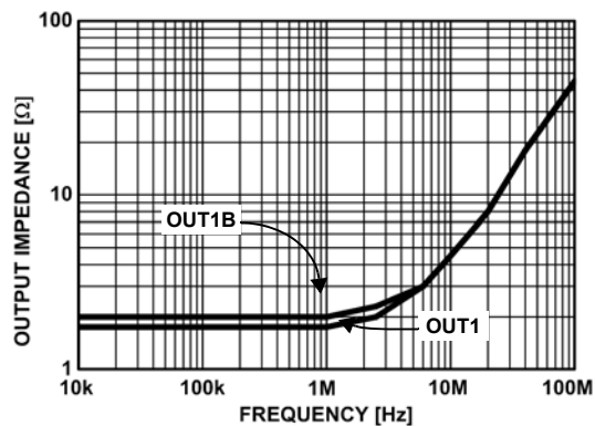
FIGURE 20. OUTPUT IMPEDANCE (ENABLED)
