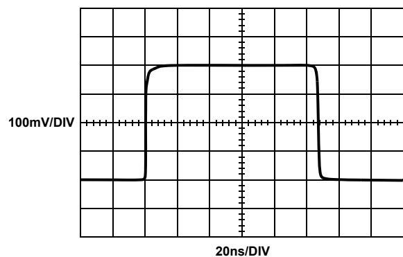
FIGURE 17. SMALL SIGNAL TRANSIENT RESPONSE
