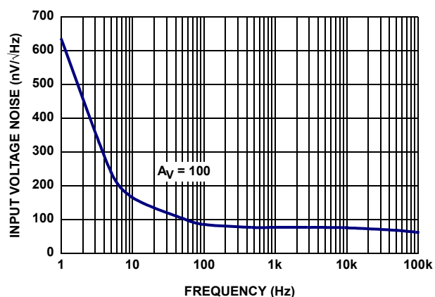
FIGURE 12. EL8172 VOLTAGE NOISE SPECTRAL DENSITY
