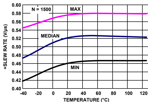
FIGURE 34. EL8172 +SLEW RATE vs TEMPERATURE, INPUT = \pm 0.015V @ GAIN + 100
