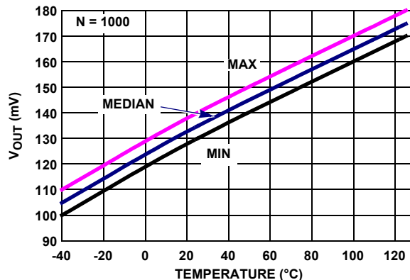
FIGURE 32. EL8172 V_{OUT} LOW vs TEMPERATURE, R_L = 1k , V_+ = 5V , V_- = \pm 2.5V
