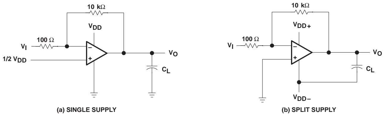
Figure 94. Gain-of-100 Inverting Amplifier
