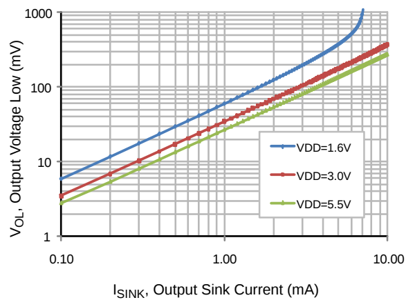
Figure 8. Output LOW vs. Output Drive Current
