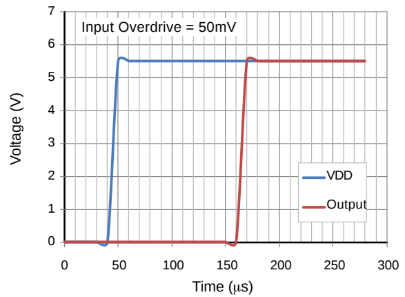
Figure 13. Power-Up Delay
