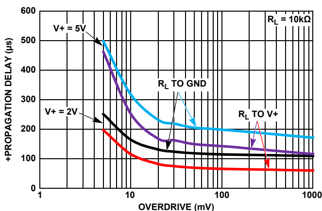
FIGURE 6. PROPAGATION DELAY vs OVERDRIVE (RISING EDGE)
