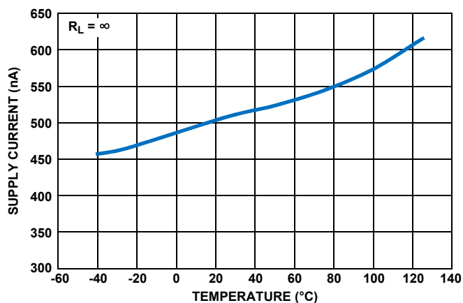
FIGURE 12. SUPPLY CURRENT vs TEMPERATURE, V+, GND = \pm 2.5V
