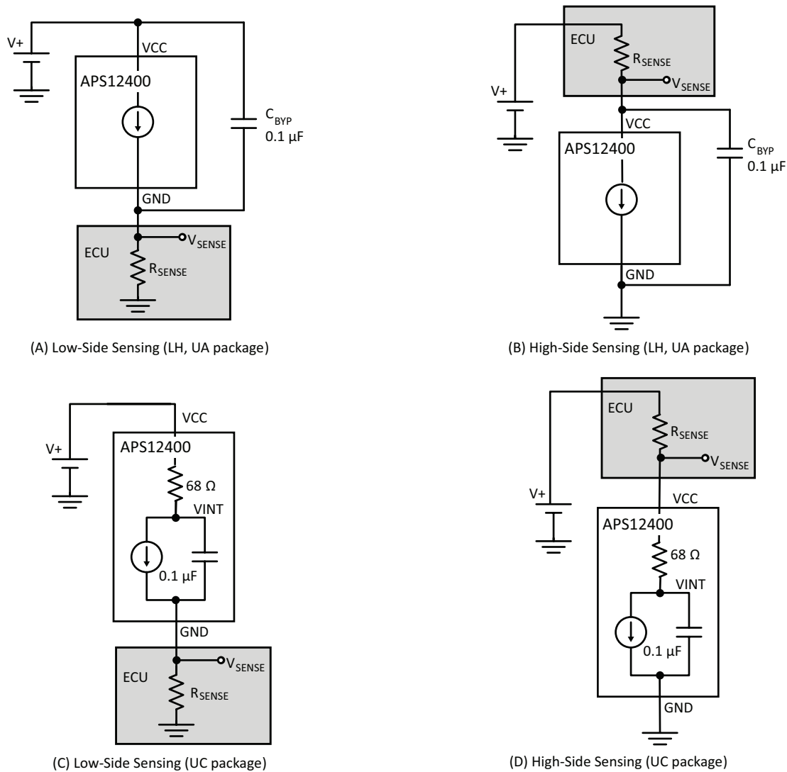
Figure 5: Typical Application Circuits
