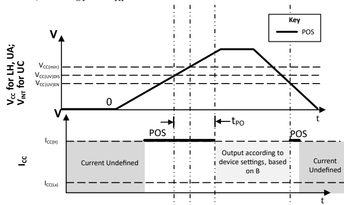
Figure 3: Power-On/UVLO Behavior
